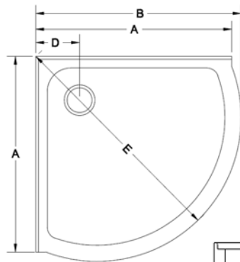
Dimensions approximatives. Approximate dimensions.
