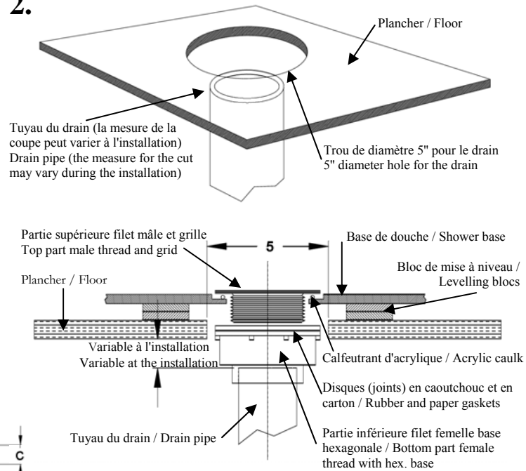
Dimensions approximatives. Approximate dimensions.
